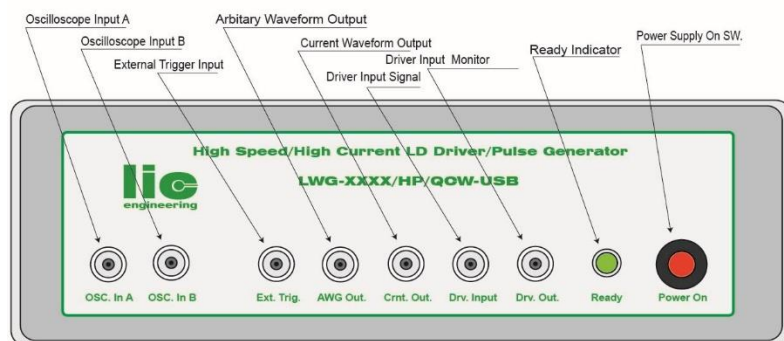
(Front Panel)
